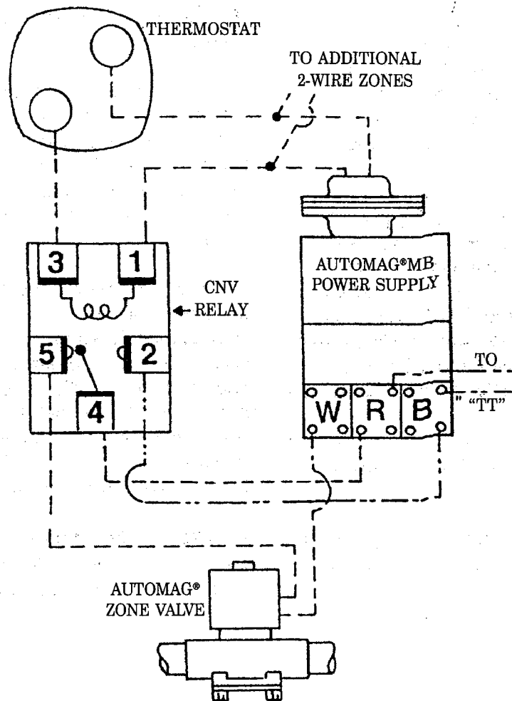
CONVERTING TO AUTOMAG® USING TWO WIRE THERMOSTATS
