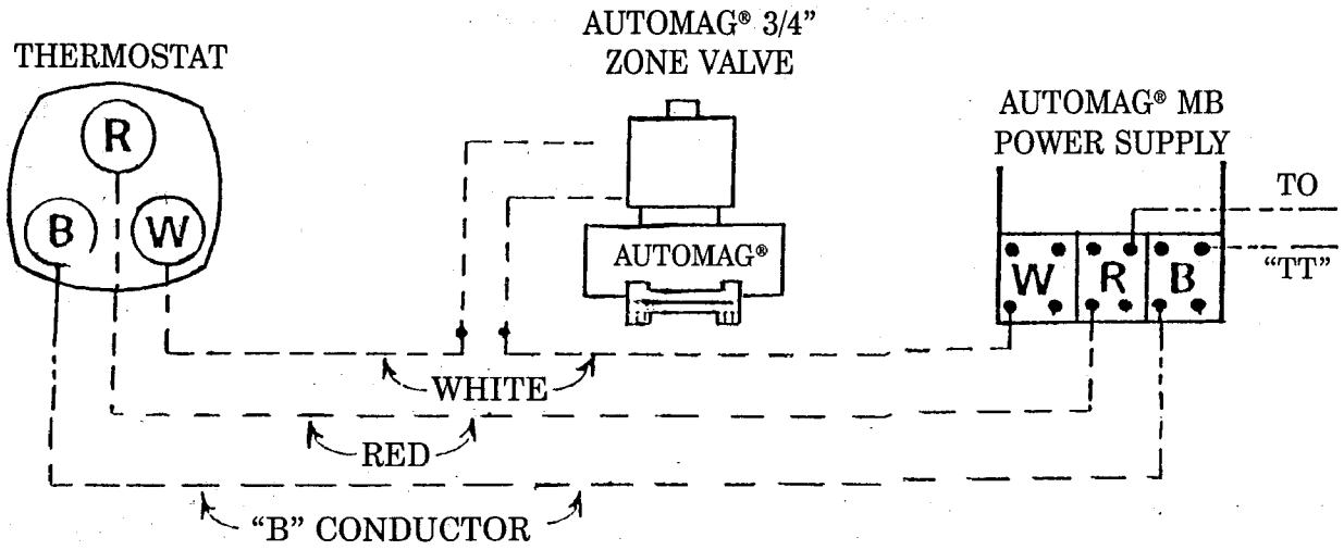
TYPICAL RESIDENTIAL SYSTEM
